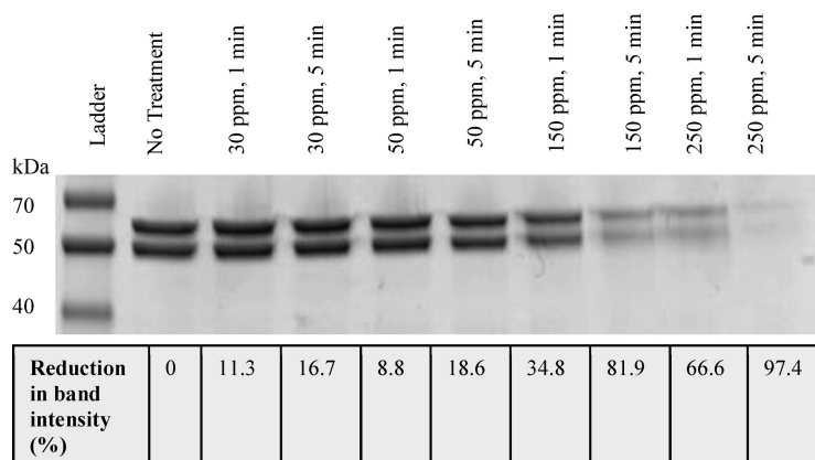
FIG 3 SDS-PAGE analysis of human NoV VLP major capsid protein. Two-microliter aliquots of purified human NoV GII.4 Grimsby VLPs were dried onto stainless steel coupons and treated with neutral electrolyzed water at various concentrations and exposure times.
